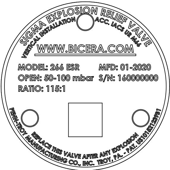
DETAIL B SCALE 1.5 : 1
